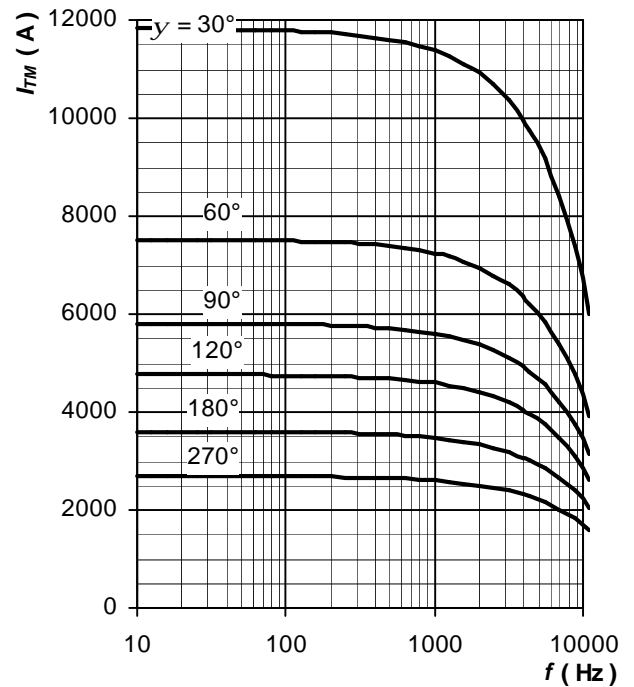
Fig. 22 Maximum on-state current vs. frequency, trapezoid waveform, T_C = 70\text{ °C} , di_T/dt = \pm 100\text{ A}/\mu\text{s} , V_R = 100\text{ V}
