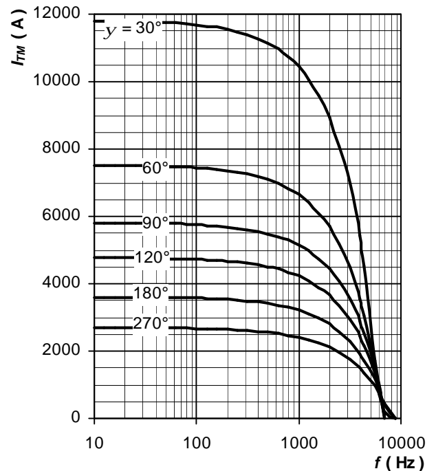
Fig. 24 Maximum on-state current vs. frequency, trapezoid waveform, T_C = 70\text{ °C} , di_T/dt = \pm 100\text{ A}/\mu\text{s} , V_R = 2/3 V_{DRM}
