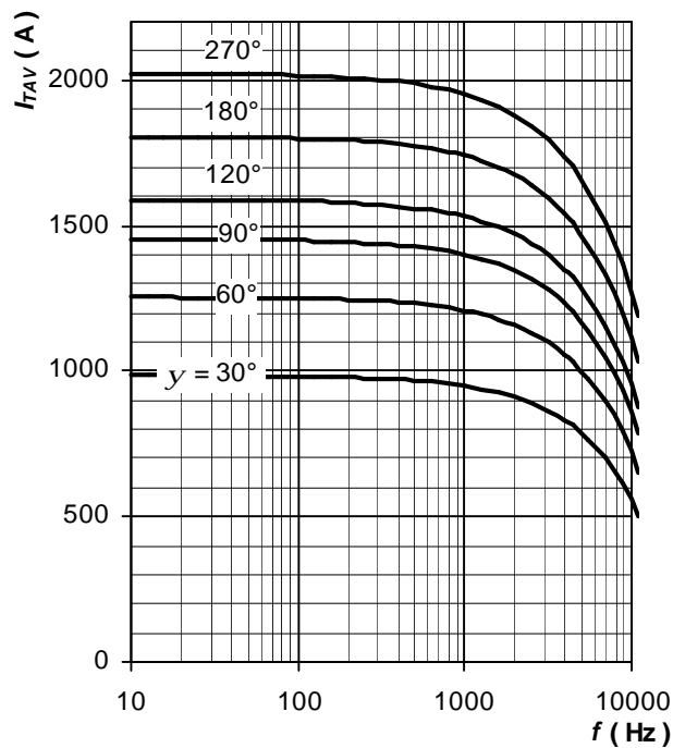
Fig. 21 Average on-state current vs. frequency, trapezoid waveform, T_C = 70\text{ °C} , di_T/dt = \pm 100\text{ A}/\mu\text{s} , V_R = 100\text{ V}
