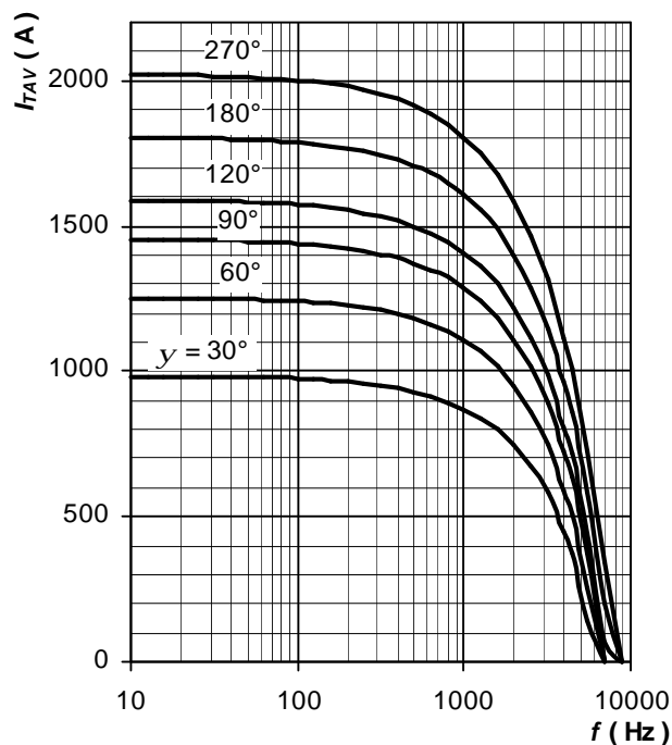
Fig. 23 Average on-state current vs. frequency, trapezoid waveform, T_C = 70\text{ °C} , di_T/dt = \pm 100\text{ A}/\mu\text{s} , V_R = 2/3 V_{DRM}
