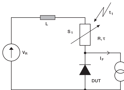
Fig. 2b Resistive commutation
